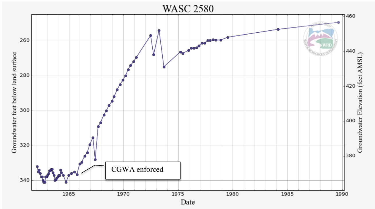
Figure 5. Representative hydrograph for The Dalles Groundwater Reservoir
