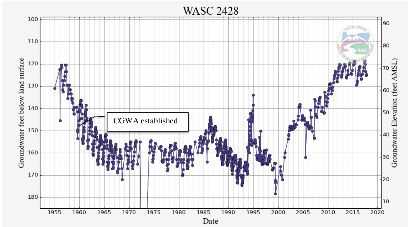
Figure 6. Representative hydrograph for The Dalles Groundwater Reservoir
