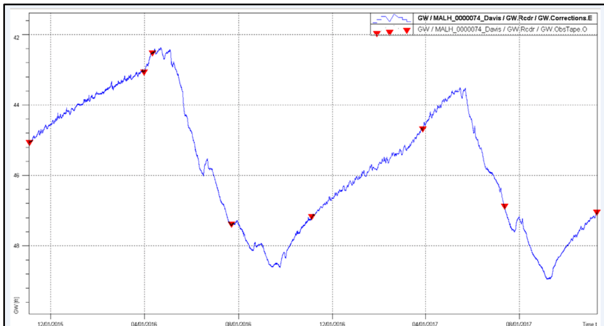
Figure 4. Water level plot of continuous recorder data (blue) and manual measurements (red)
