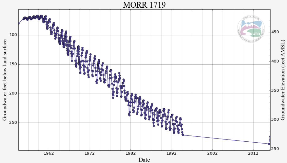
Figure 9. Representative long-term hydrograph for Ordnance Deep Basalt aquifer
