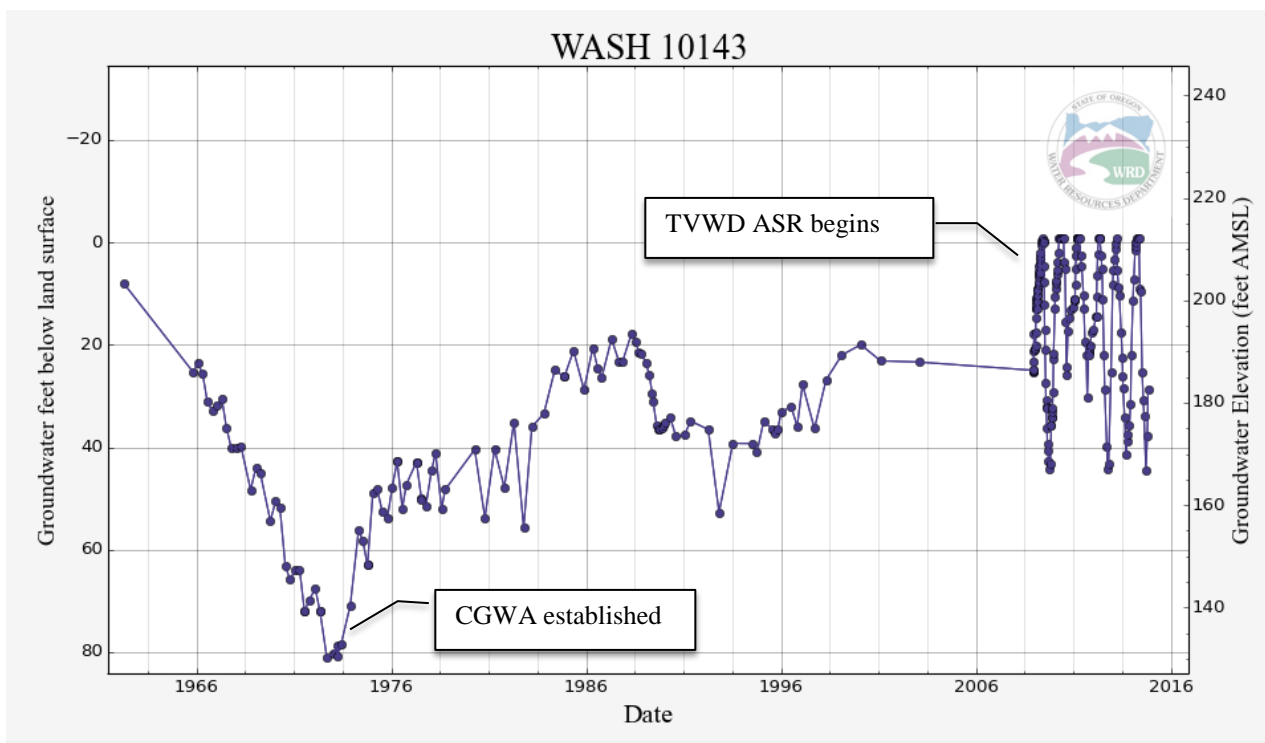
Figure 8. Hydrograph showing Cooper-Bull Mountain CGWA well response to ASR
