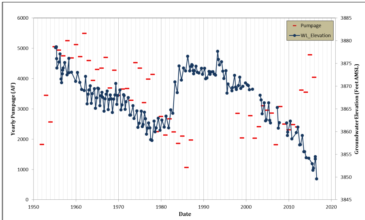
Figure 2. Total water use data from permitted wells in Cow Valley CGWA show an inverse relationship to groundwater elevations
