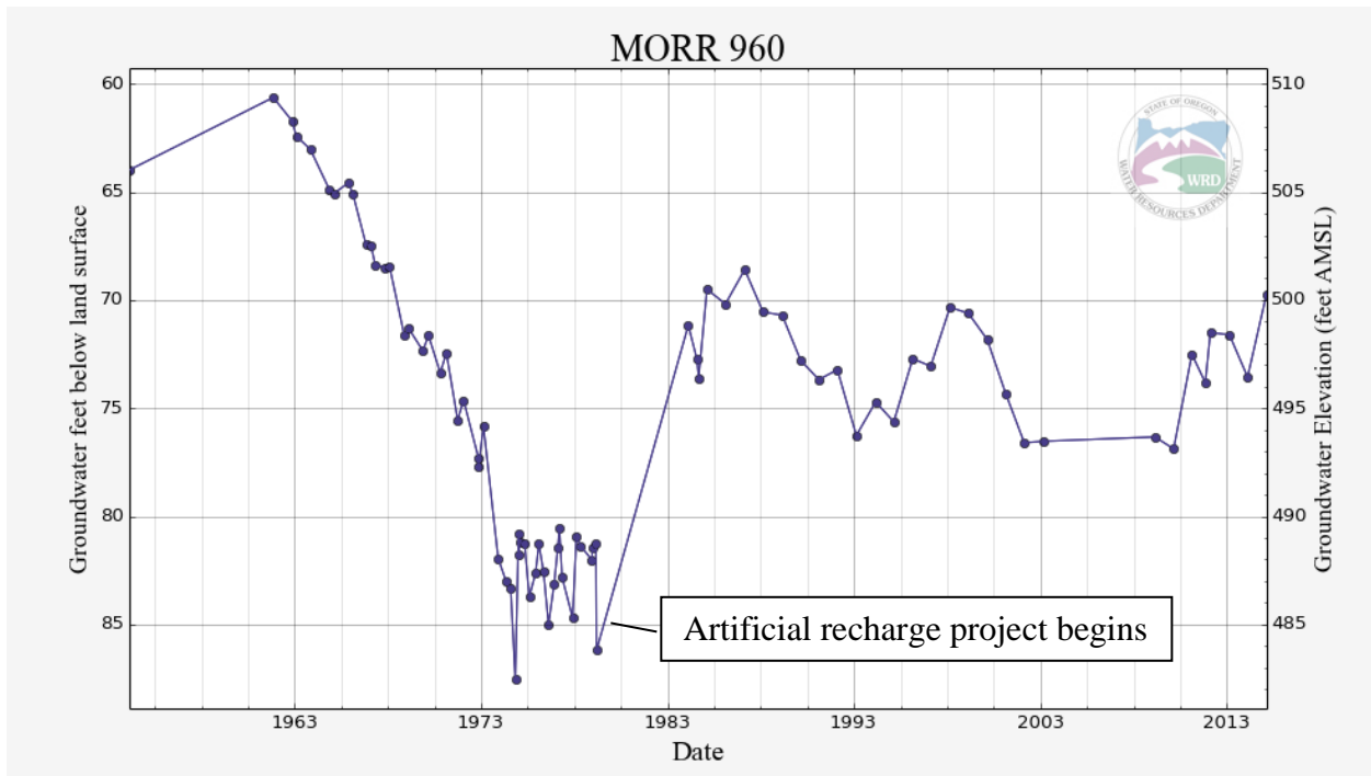
Figure 11. Representative long-term hydrograph for Ordnance Gravel CGWA
