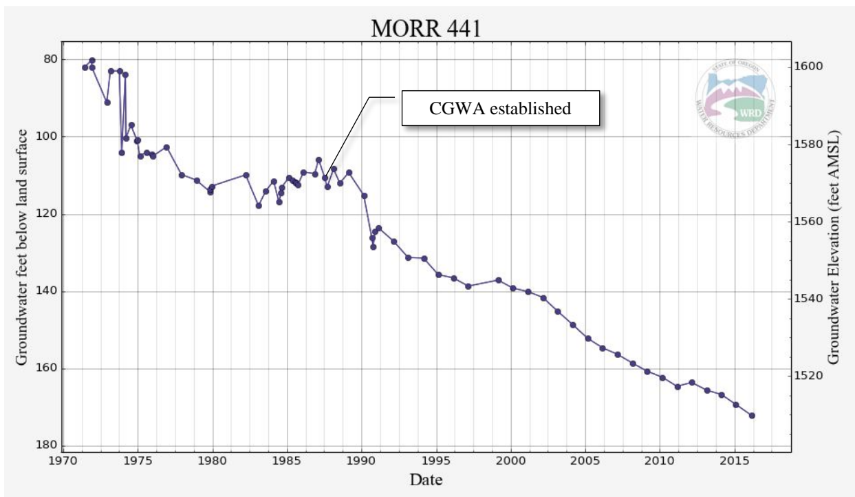
Figure 14. Representative hydrograph for Butter Creek CGWA South Subarea
